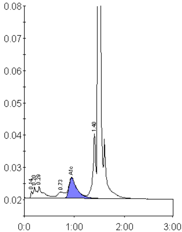
Peak table - ID: 10550772
